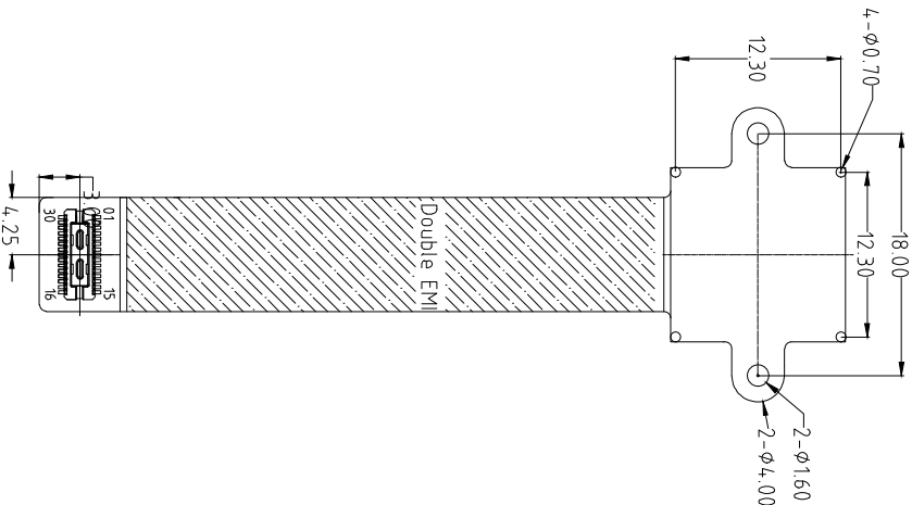
BOTTOM VIEW
